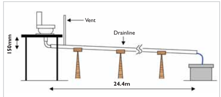
Figure 1 Laboratory Setup
